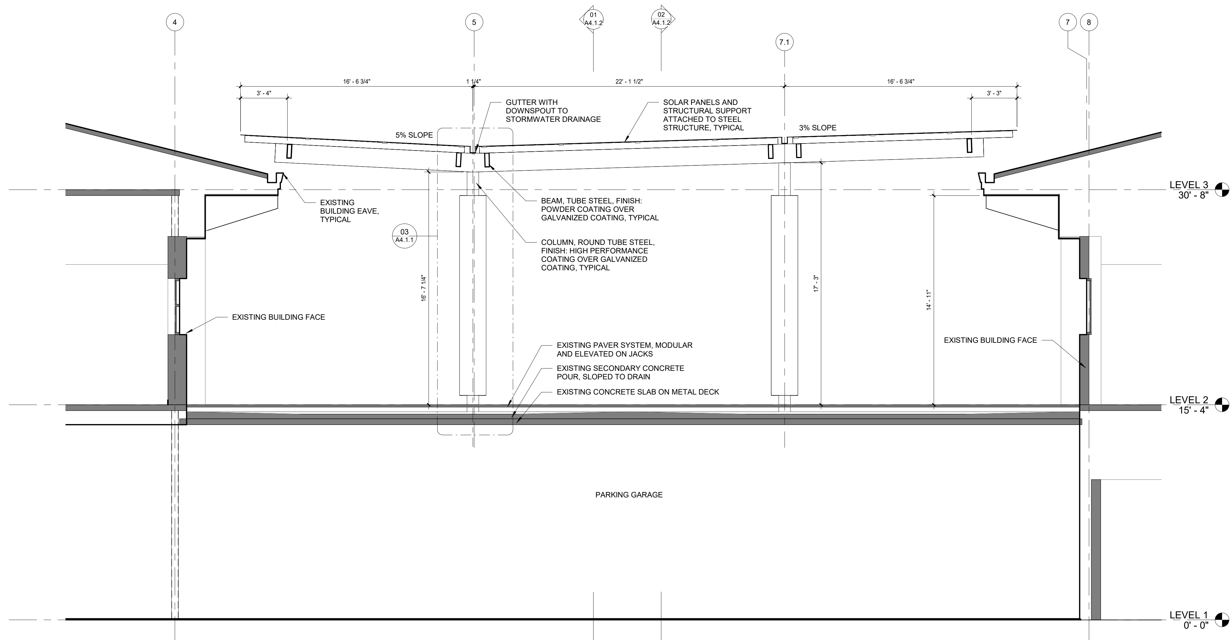
01 BUILDING SECTION 1/4" = 1'-0"
